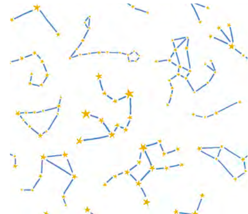
29864 Z Constellations
